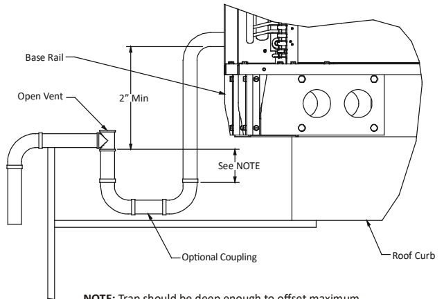
DRAIN PAN (SIDE VIEW) FIGURE 9
