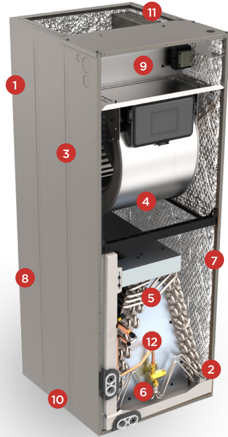
JHC Single Piece Air Handler
