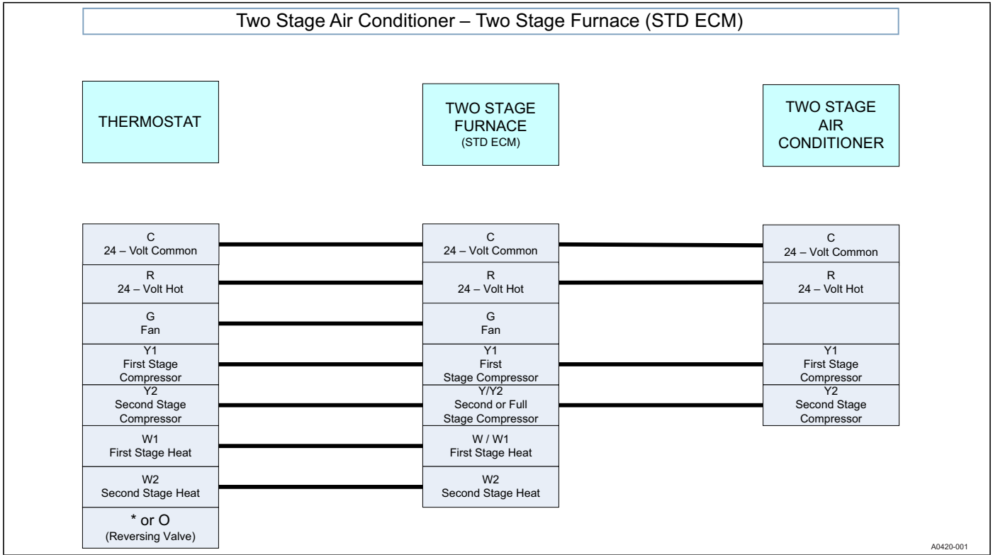
FIGURE 12: Thermostat Chart - Two Stage AC with Two Stage Standard ECM Furnaces
