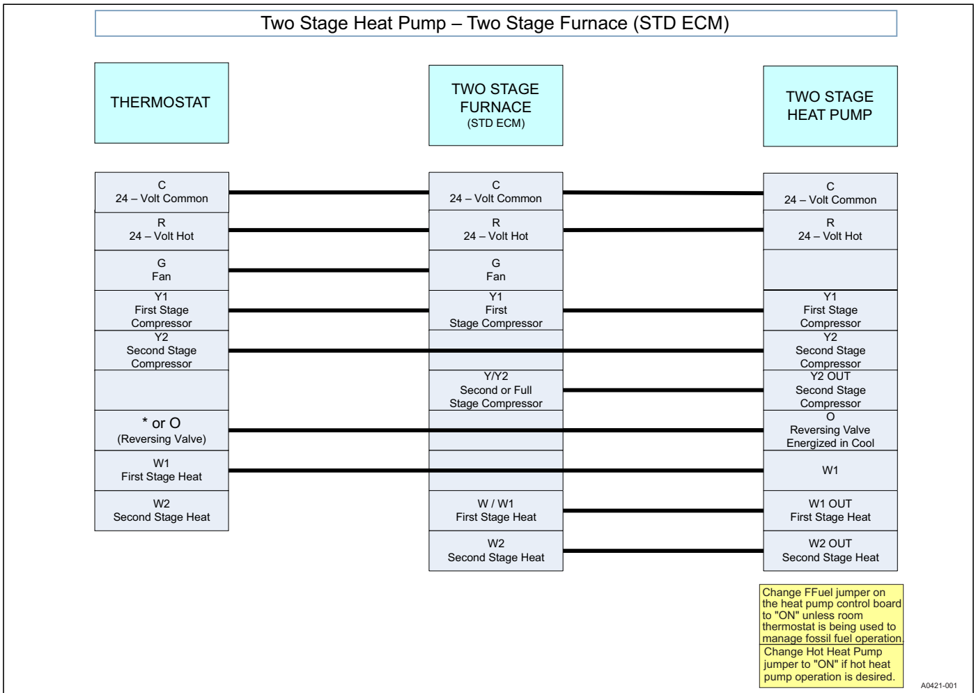
FIGURE 13: Thermostat Chart - Two Stage HP with Two Stage Standard ECM Furnace
