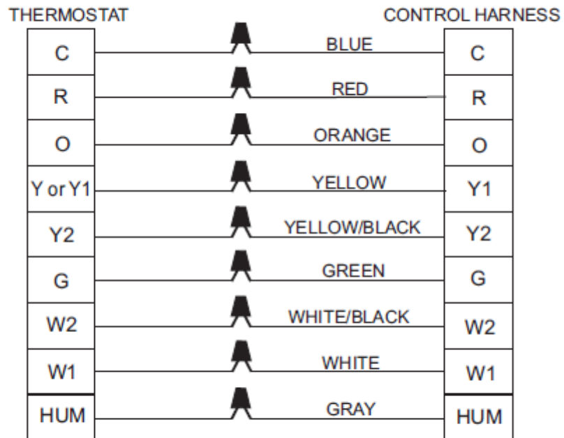
FIGURE 6: Typical Field Control Wiring Diagram For Heat Pump Models
