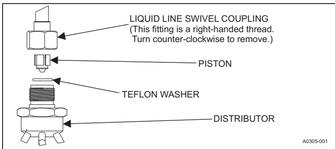
FIGURE 23: Piston Installation
