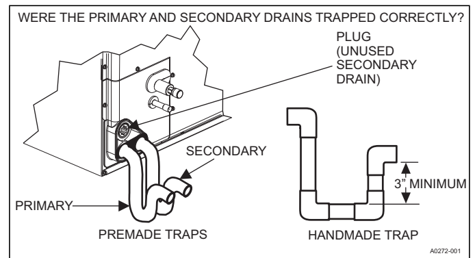
FIGURE 32: Drain Traps
