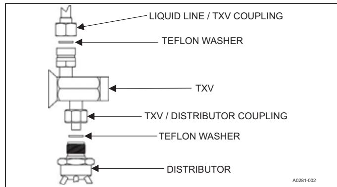
FIGURE 24: TXV Installation
