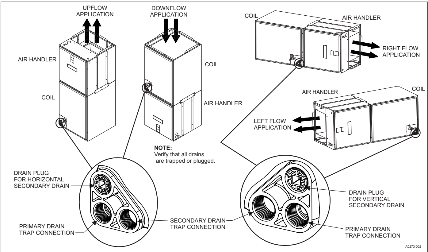
FIGURE 34: Location of Coil Trapped and Plugged Drain Connections with Modular Air Handler
