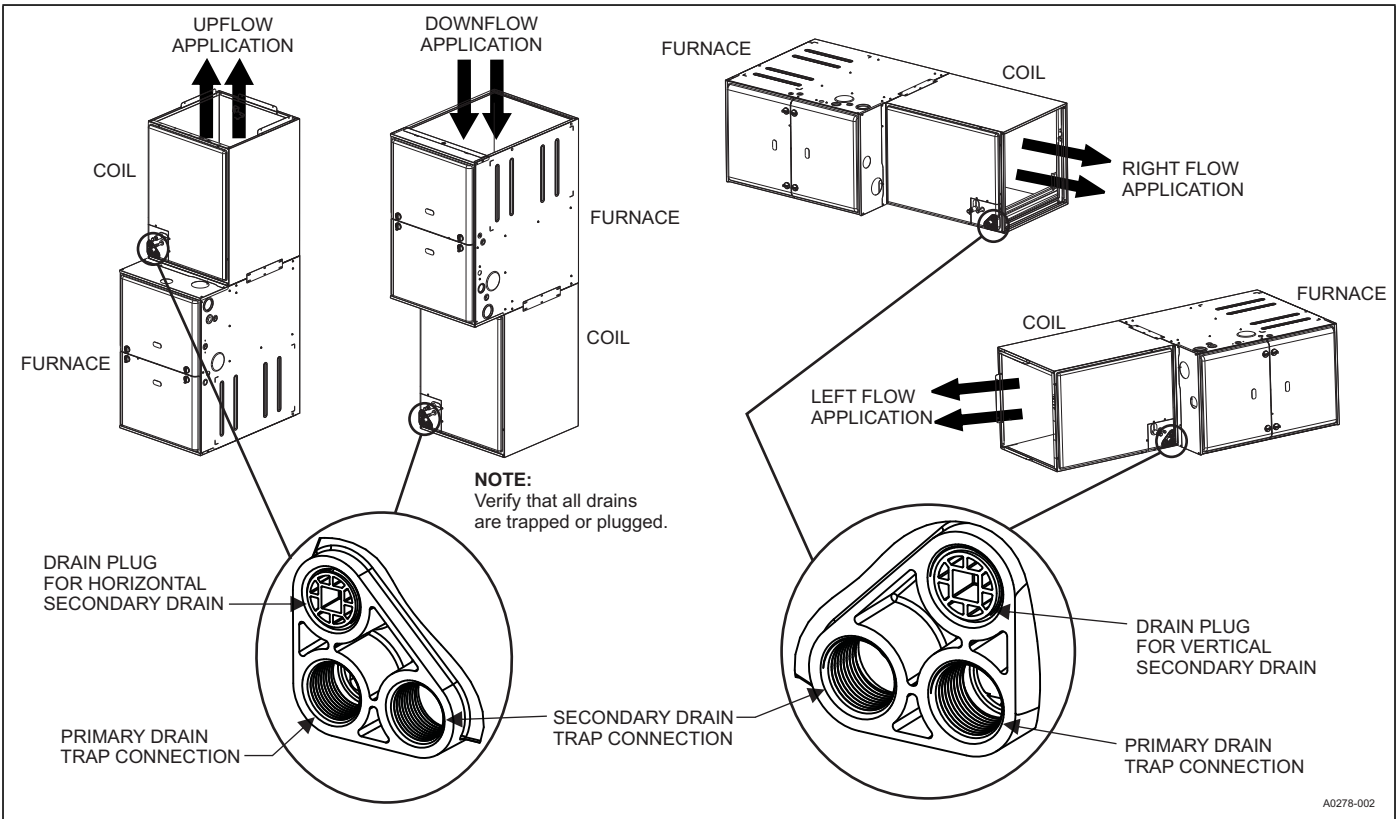
FIGURE 33: Location of Coil Trapped and Plugged Drain Connections with Furnace
