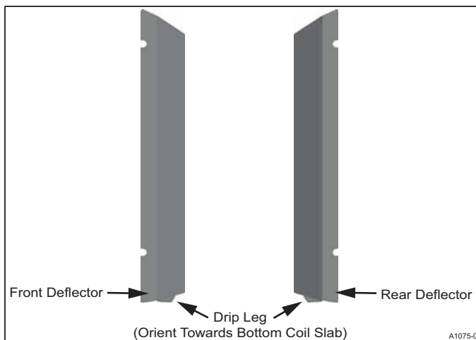
FIGURE 11: CM60C Horizontal Right Condensate Deflectors
