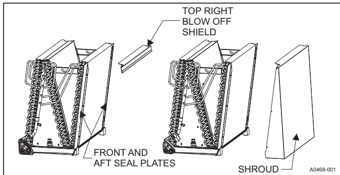
FIGURE 20: Diverter Shroud Installation
