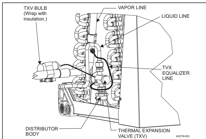
FIGURE 25: TXV Bulb and Equalizer line Installations
