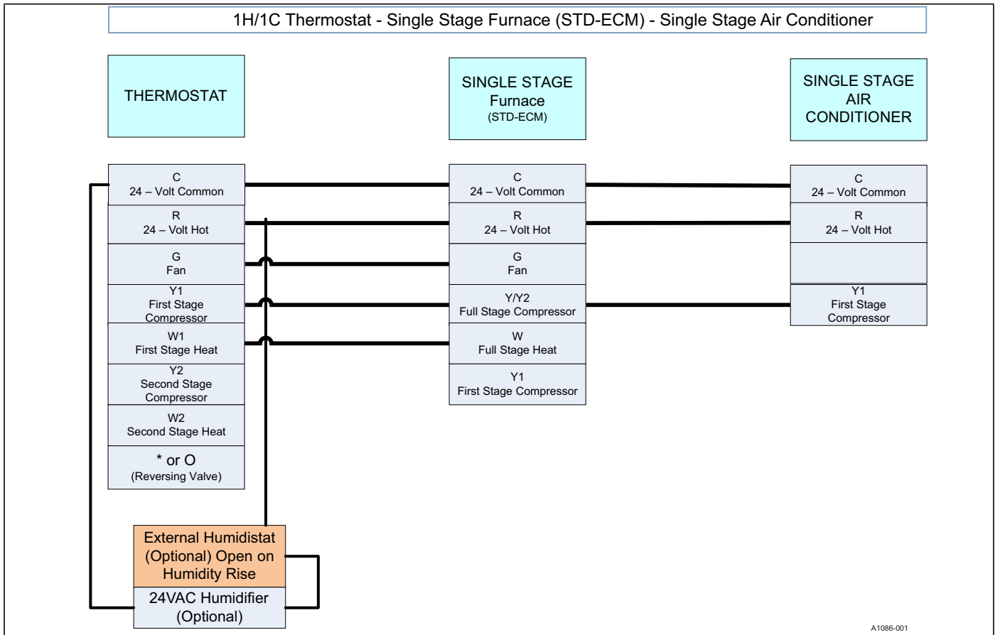
FIGURE 14: Thermostat Chart - 1H/1C - Single Stage Furnace (STD-ECM) - Single Stage Air Conditioner
