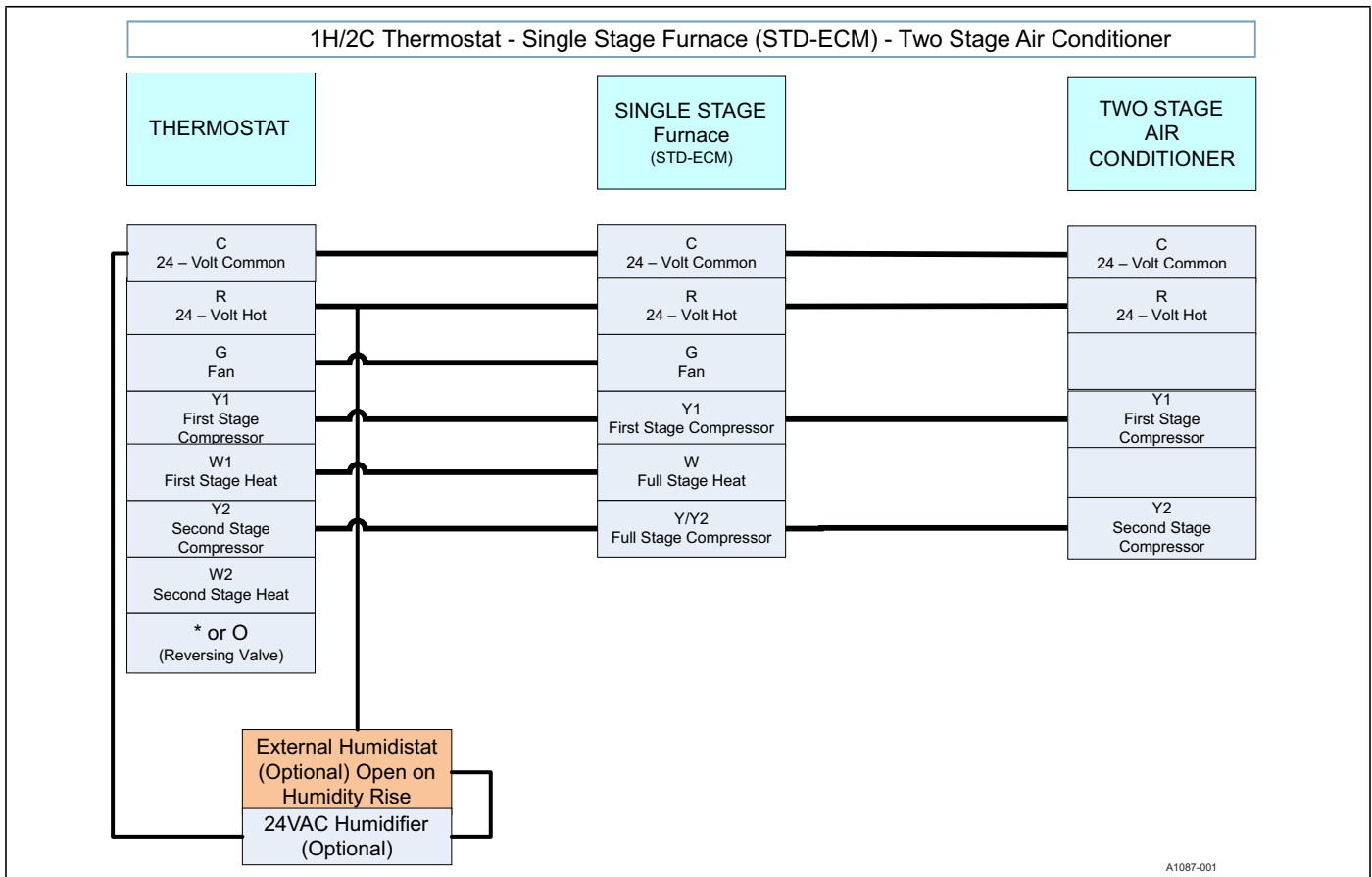
FIGURE 15: Thermostat Chart - 1H/2C - Single Stage Furnace (STD-ECM) - Single Stage Air Conditioner
