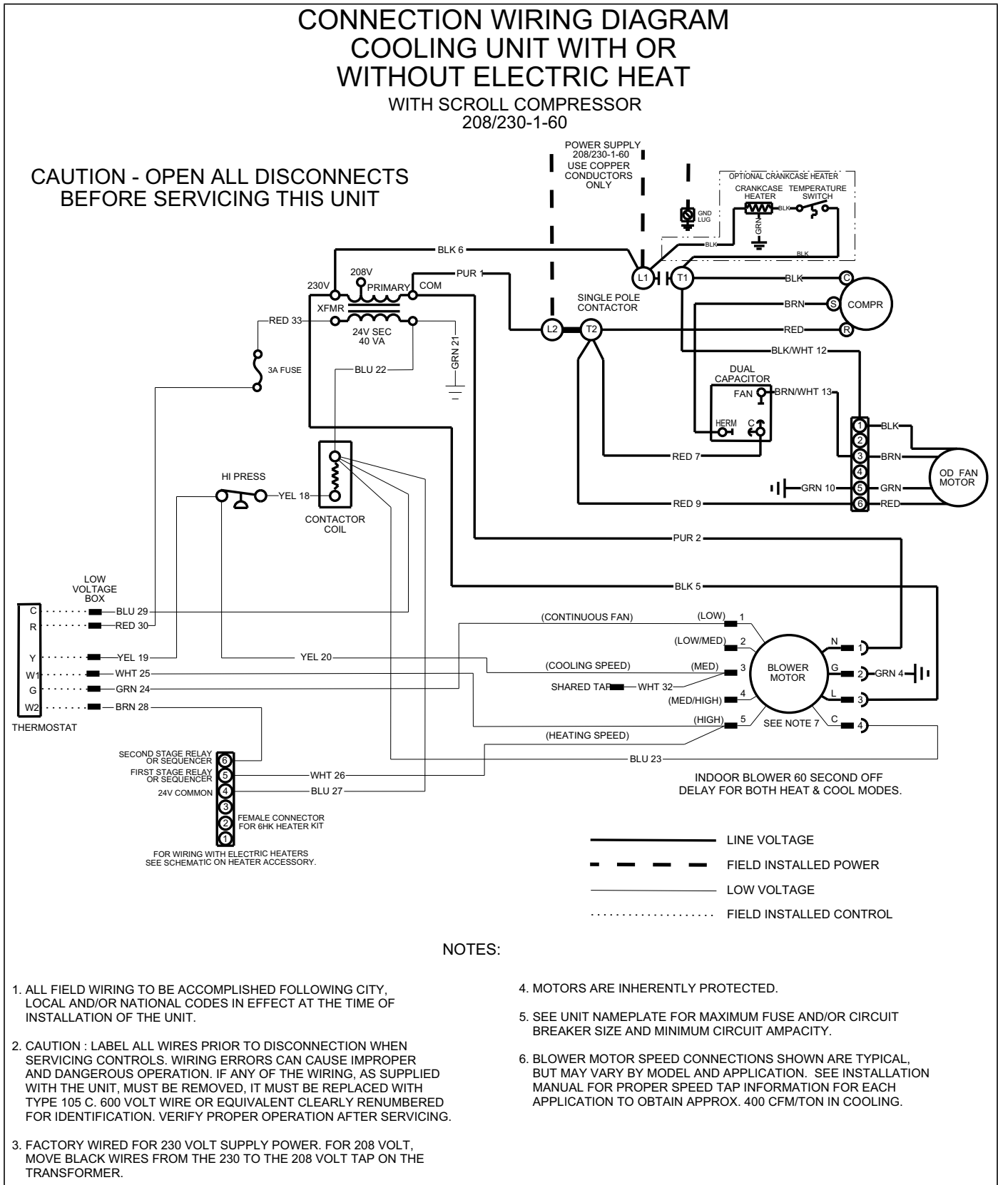
Figure 10: Connection Wiring Diagram
