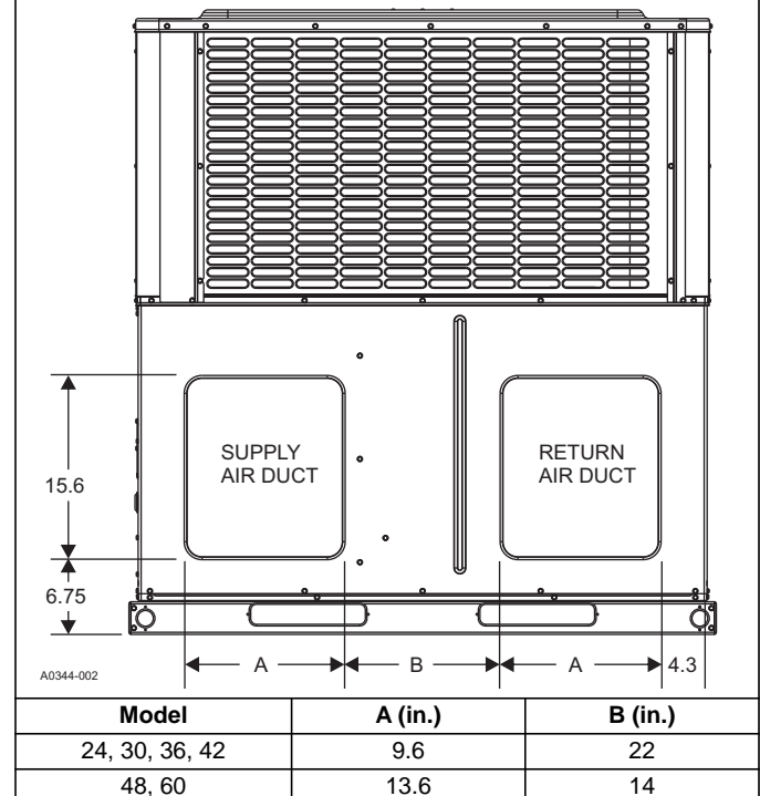
Figure 5: Rear Duct Dimensions (in.)
