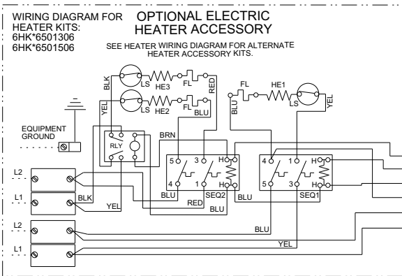
Figure 11: Ladder Wiring Diagram
