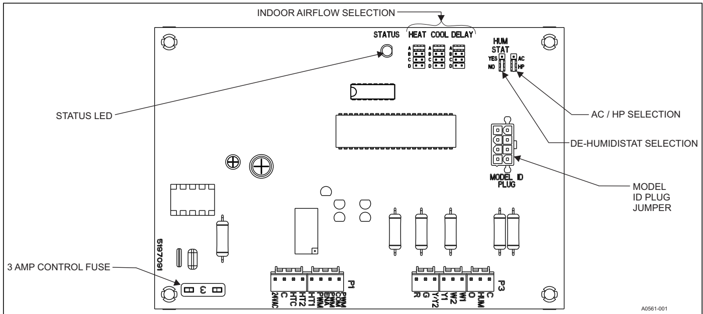
Figure 10: Blower Control
