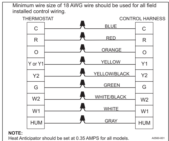
Figure 6: Typical Field Control Wiring Diagram for Heat Pump Models
