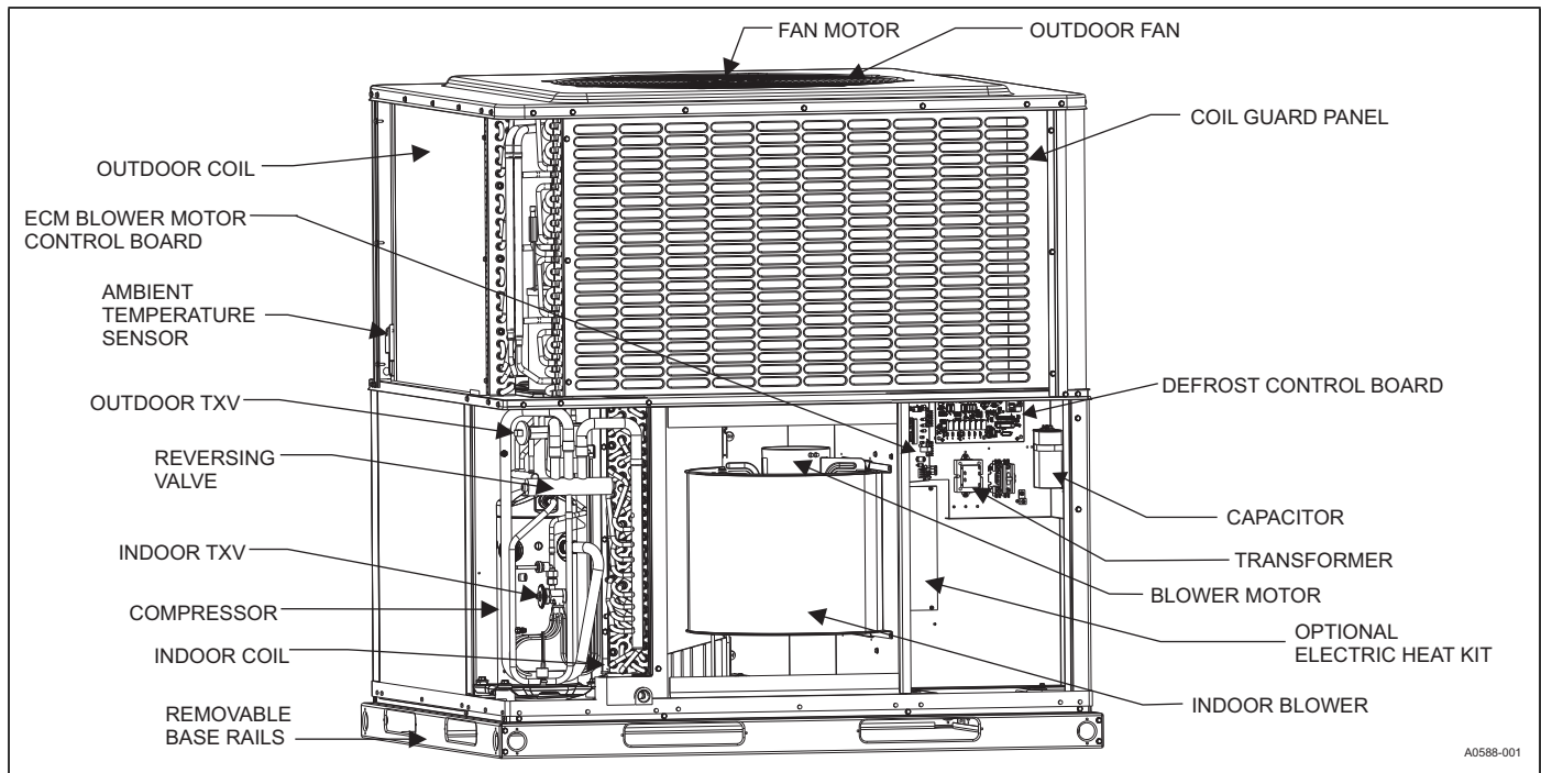
Figure 1: Component Location
