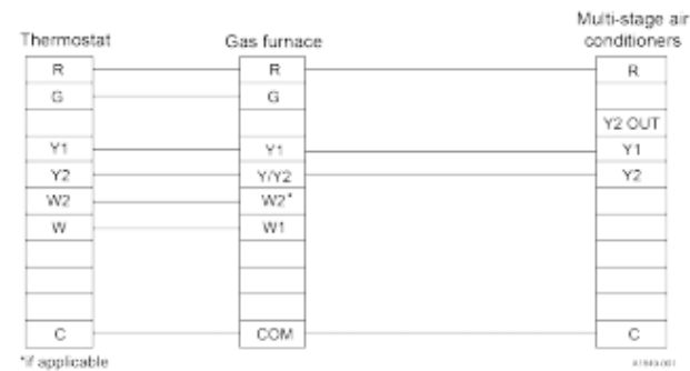
Figure 20: Standard ECM furnace and premium multi-stage AC
