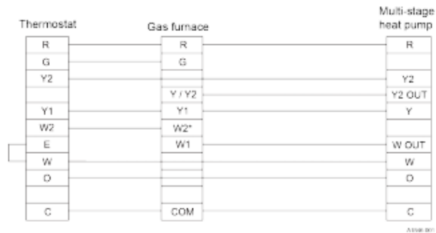
Figure 19: Standard ECM furnace and single-stage AC
