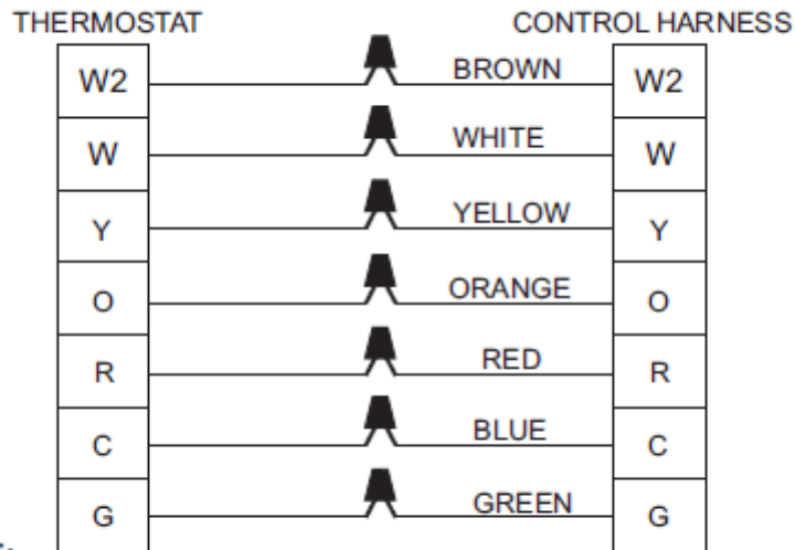
FIGURE 6: Typical Field Control Wiring Diagram For Gas Heat - AC Models
